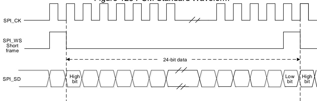
Figure 123 PCM Standard Waveform
