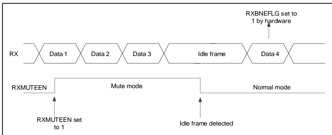
Figure 92 Idle Bus Exit MuteMode
