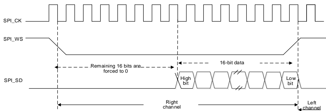
Figure 121 Under LSB Alignment Standard (extending from 16 bits to 32 bits)
