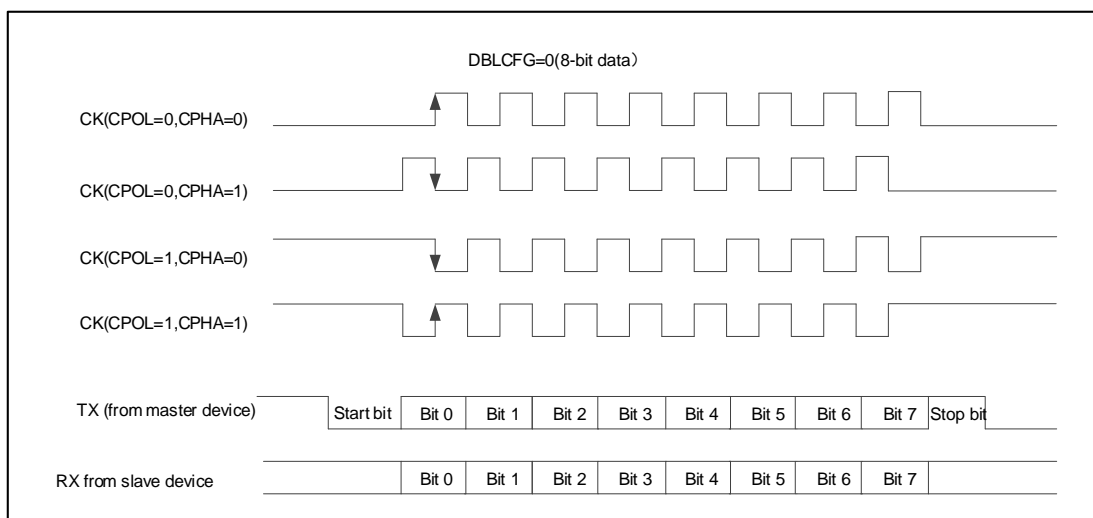
Figure 95 USART Synchronous Transmission Timing Diagram (DBLCFG=0)
