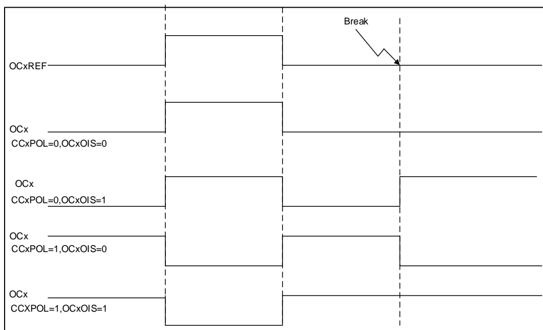
Figure 64 Breaking Event Timing Diagram
