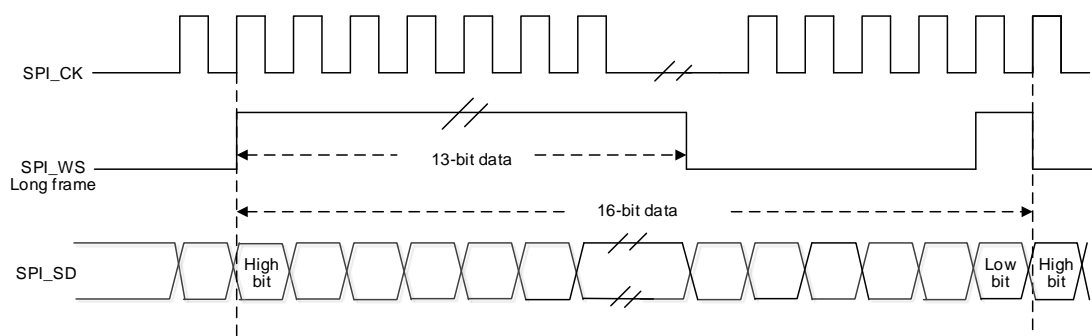
Figure 122 PCM Standard Waveform
