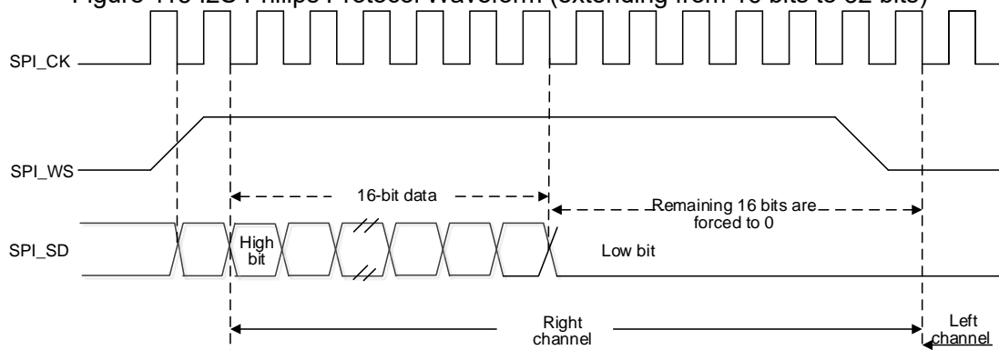
Figure 115 I2S Philips Protocol Waveform (extending from 16 bits to 32 bits)
