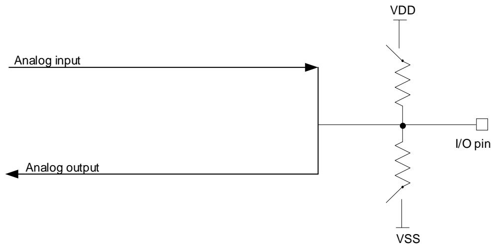
Figure 21 Analog Function I/O Structure
