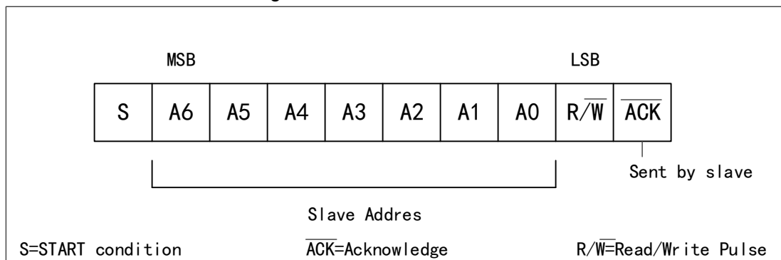
Figure 82 7-bit Address Format
